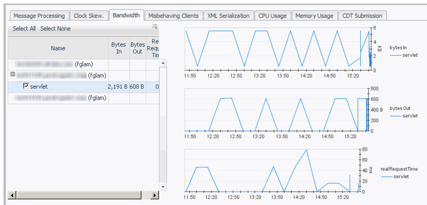
Figure 8. Bandwidth tab
