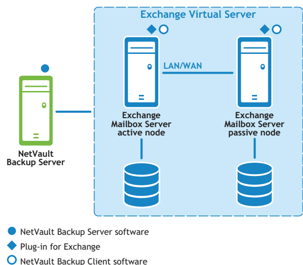
Figure 5. CCR deployment
