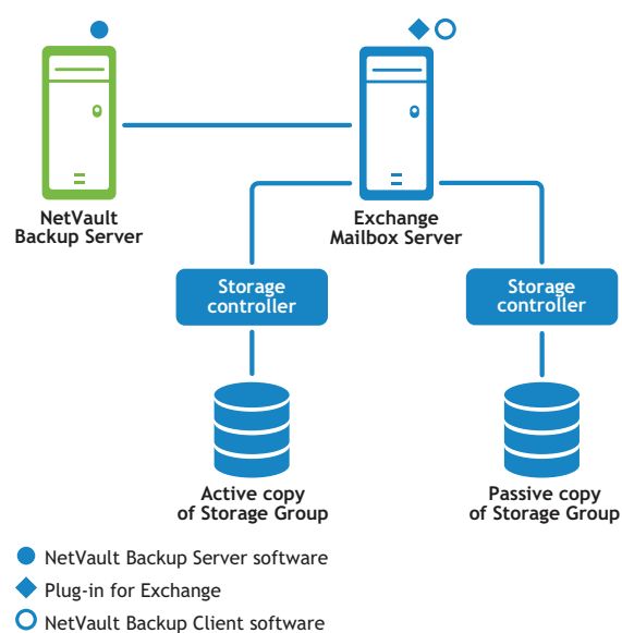
Figure 3. LCR deployment
