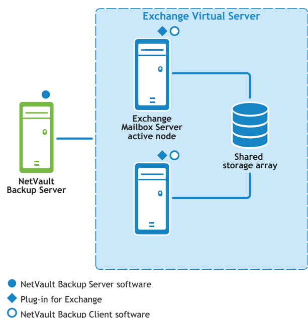
Figure 4. SCC deployment
